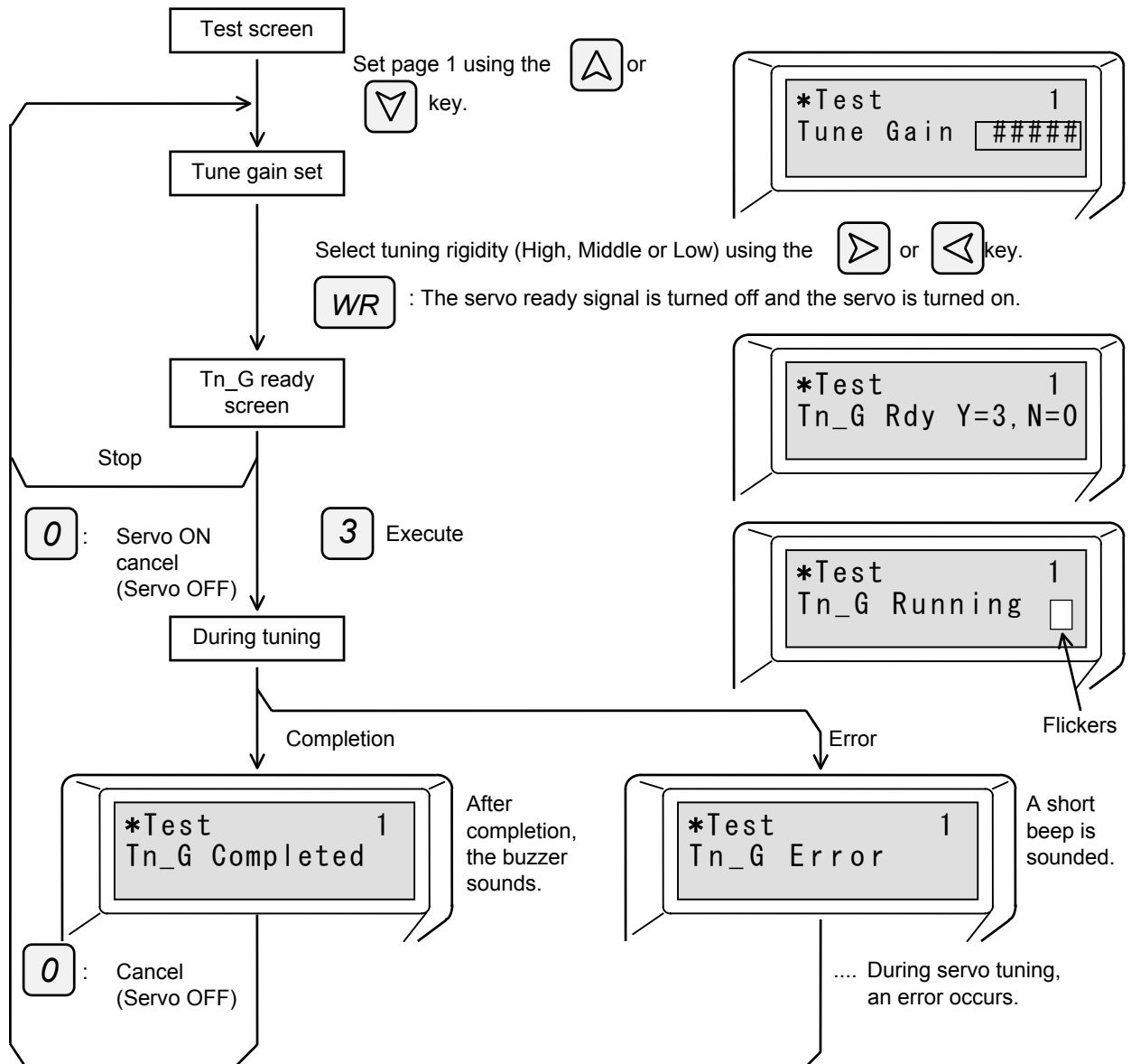
Fig. 7-12 Offline automatic Tuning Operation
