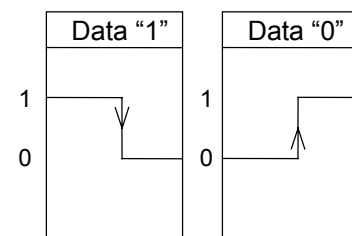
Manchester code
