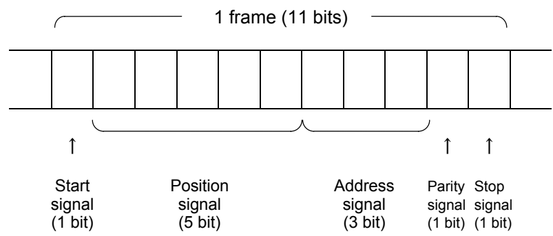
Fig. 9-9-1 (1) Start-stop Synchronization (9600bps) Frame Configuration (ABS-E.S1)
