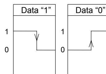
Manchester code
