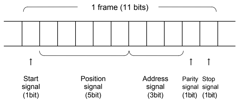
Fig. 9-7-1 (1) Frame Configuration of Start-stop Synchronization (9600 bps)(ABS-E)
