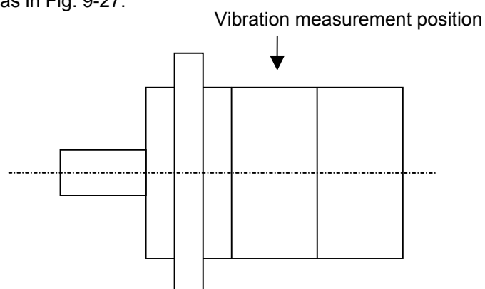
Fig. 9-27 Vibration Measurement
