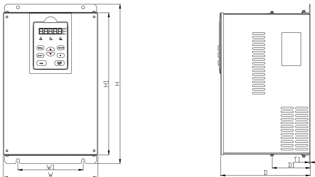
Рис. 2-3 FV100-4T-0450G ~ FV100-4T-0900G
