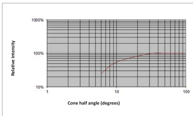
Figure 3: Optical output power vs. half angle
