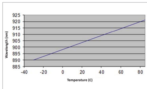
Figure 4: Wavelength vs. temperature
