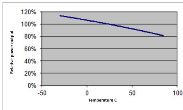
Figure 2: Optical output power vs. temperature
