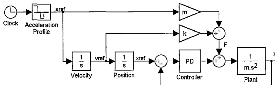
Figure 3: Mass feedforward implementation.
