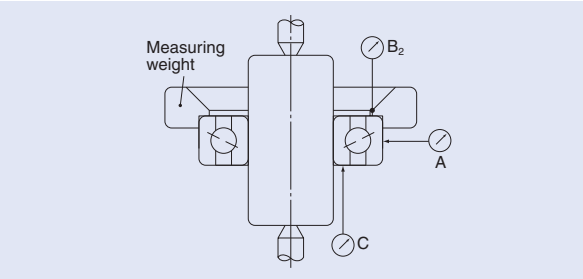
Fig. 7.1 Measuring Methods for Running Accuracy
