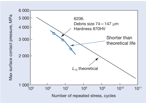
Fig. 1.3 Life Test Result under Contaminated Lubrication Condition
