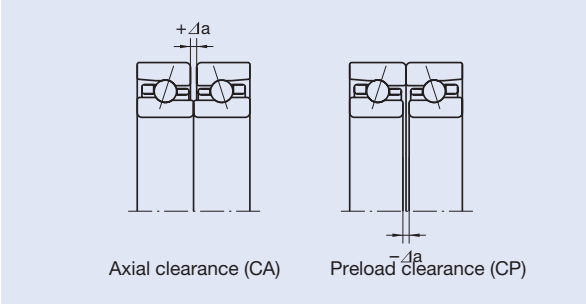
Fig. 4.9 Special Clearance
