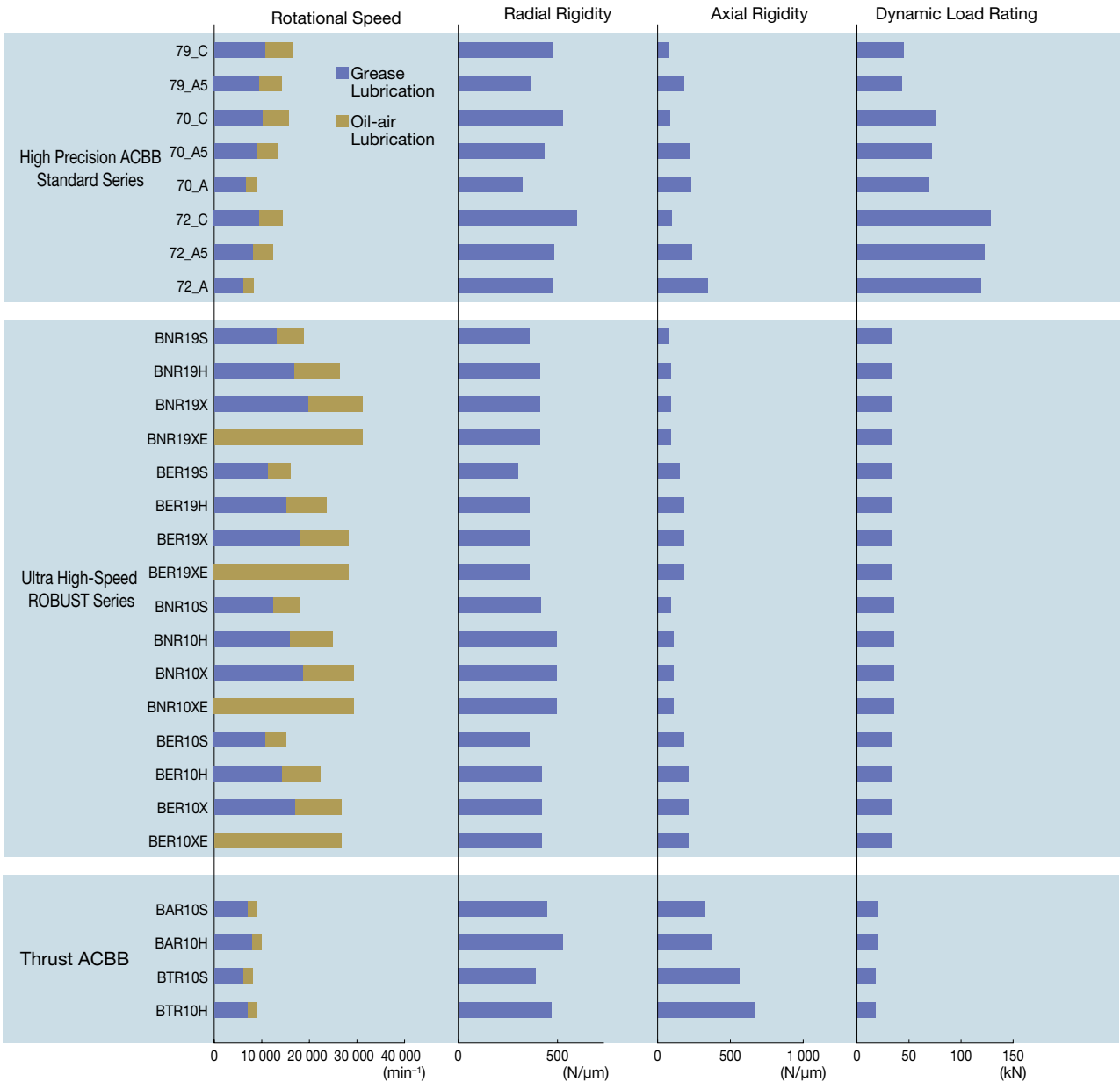
Performance Comparison of Each Type of Bearing (bore size 70 mm, DB combination, L preload)
