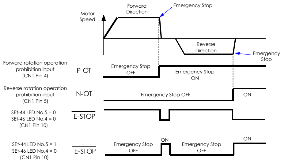
Fig 6.15 Emergency Stop
