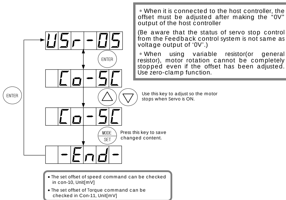
Fig 4.10 Manual Adjustment of Speed Command Offset (In case of the manual adjustment of torque command offset , " Co-tC" is displayed.)
