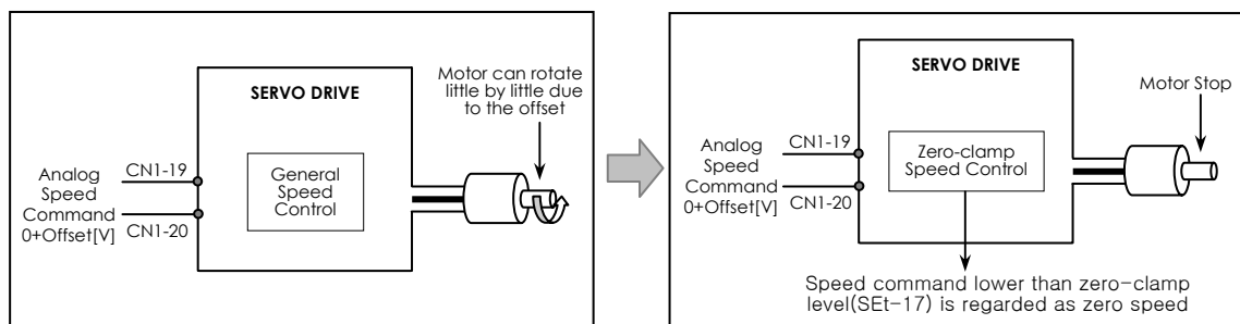
Fig 6.9 Using the Zero-Clamp Speed Control
