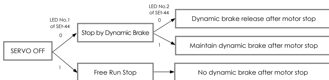
Fig 6.14 Selection of Stop Method
