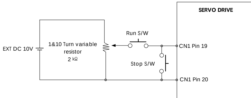
Fig 3.7 Speed Command Analog Input
