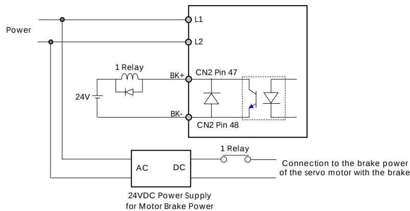
Fig 7.5 Using Brake Relay
