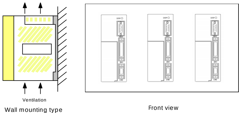
Fig 2.6 Installation of Servo Drive (Wall mounting type)
