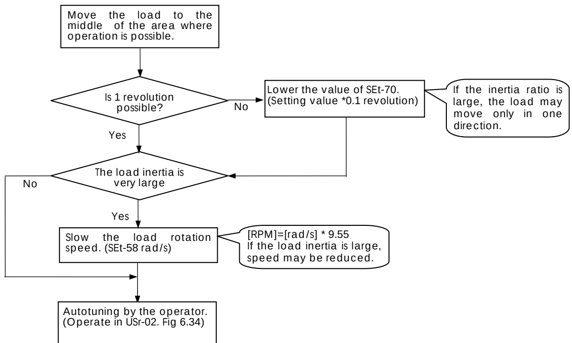
Fig 3.8 Autotuning Procedure
