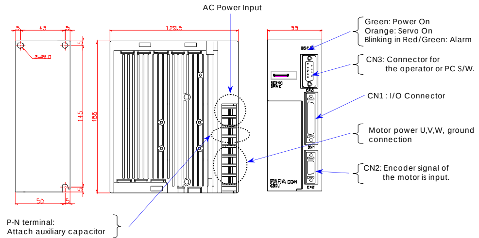
Fig 1.2 Outline Dimension (CSDJ-A3C,A5C,01B,02B,04B)
