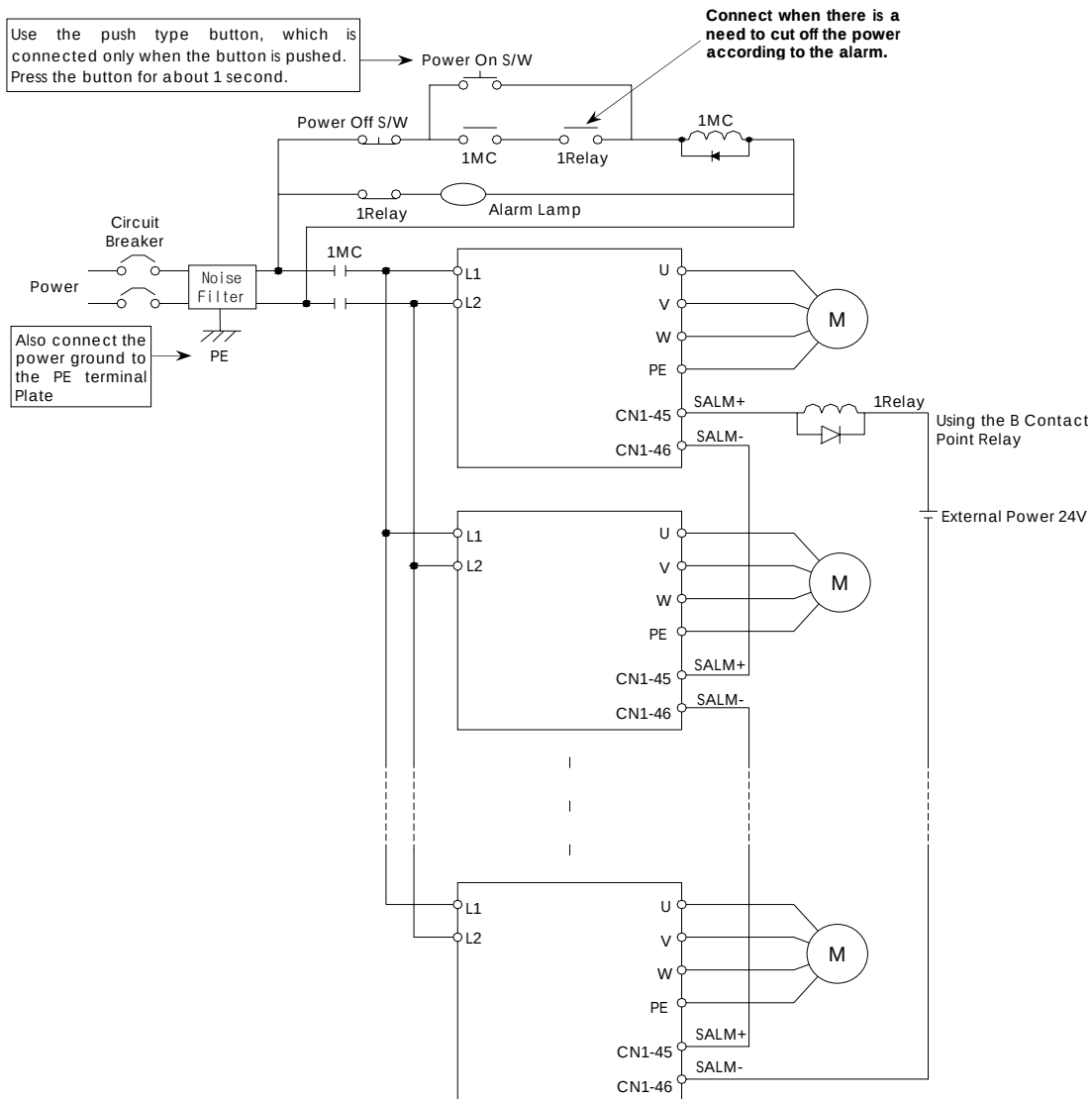
Fig 3.2 Power Supply Method for Multi-Servo Drive Connection
