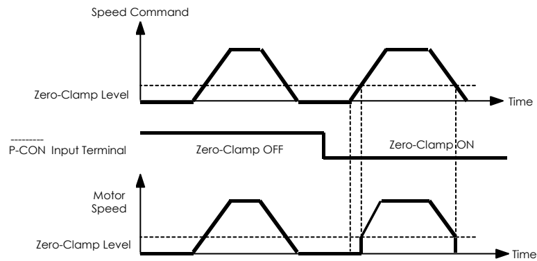
Fig 6.10 Zero-Clamp Operation
