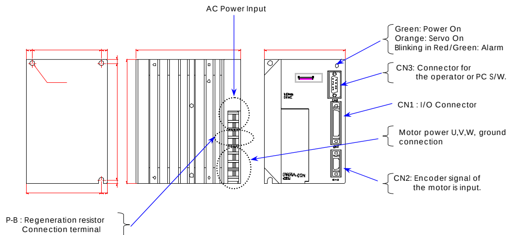
Fig 1.3 Outline Dimension (CSDJ-02C,06B,10B)
