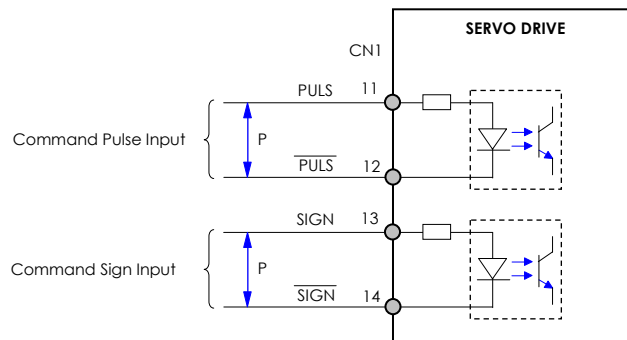
Fig 6.17 Position Command Input Terminal
