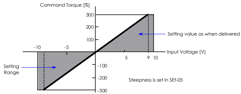
Fig 6.31 Input Voltage and Command Torque
