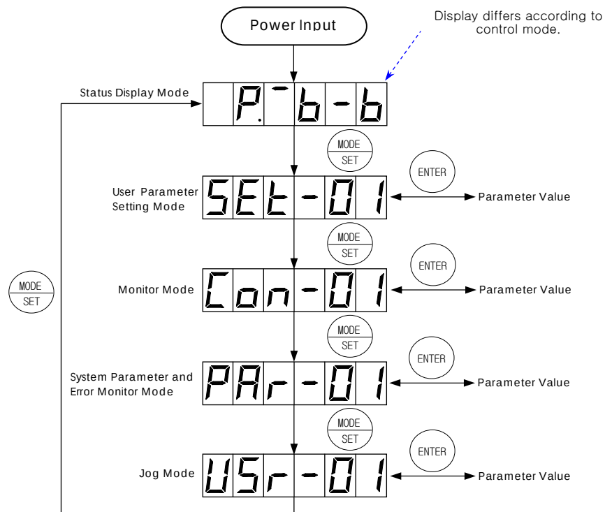
Fig 4.2 Mode Switching
