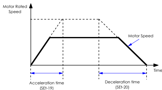
Fig 6.13 Definition of Acceleration/Deceleration Time
