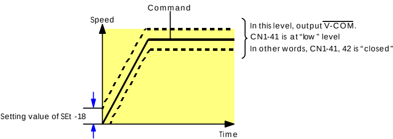
Fig 6.11 Width of Speed Coincidence Output Signal
