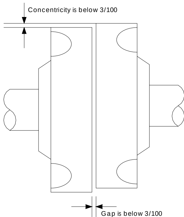
Fig 2.5 Coupling
