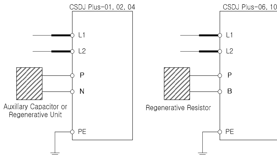
Fig 7.9 Regeneration Resistor and Regeneration Unit Connection
