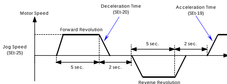
Fig 3.10 Operation Pattern of the Test Run
