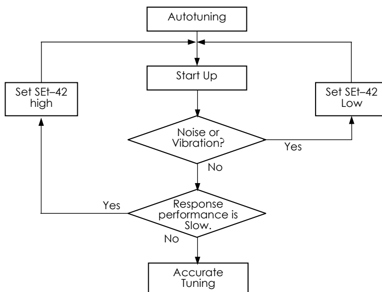
Fig 6.34 Gain Tuning
