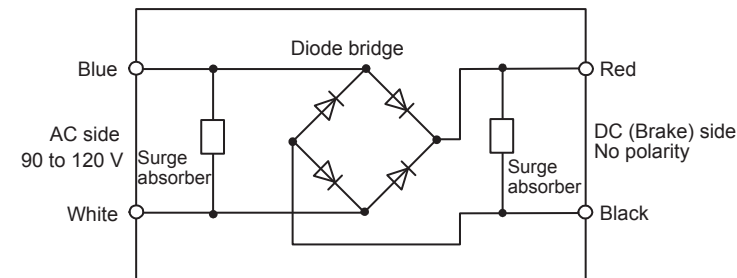
(b) Internal Circuit for 100 VAC Brake Power Supply Model: LPDE-1H01
