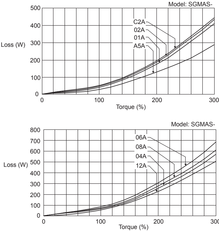
(b) SGMAS servomotor, 100/200V
