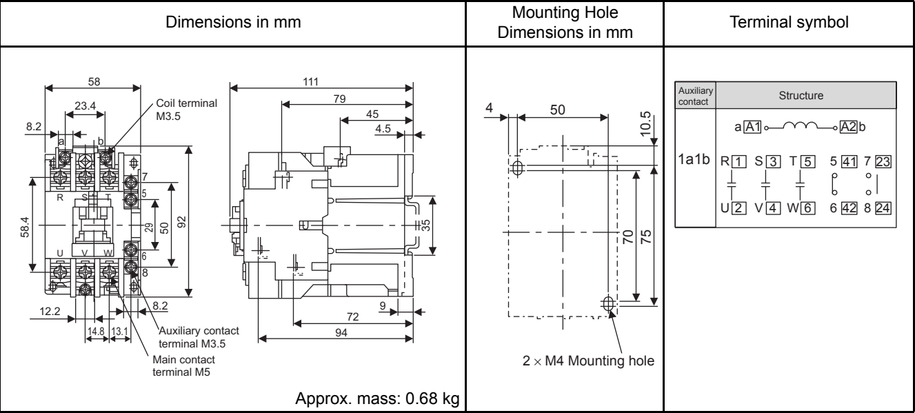
(c) Model: HI-25J and HI-35J
