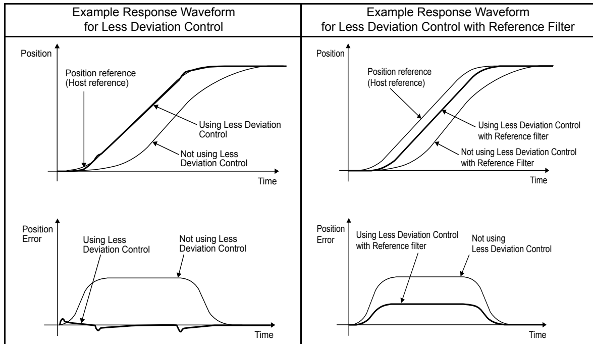
Example Response Waveforms for Less Deviation Control
