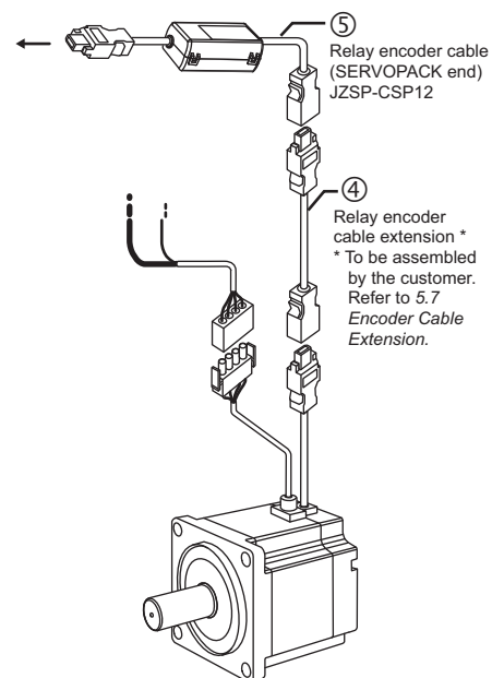
750 W, 1.5 kW SGMP5-08, 15 Servomotors
