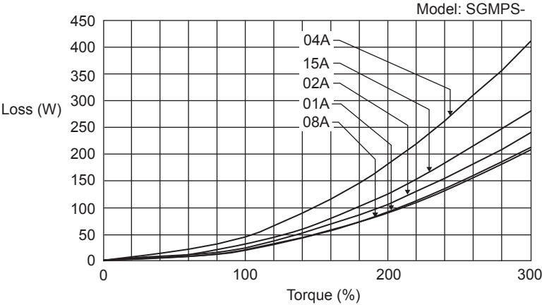
(c) SGMPS servomotor, 100/200 V
