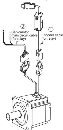
SGMP5-08, 15 Servomotor for 750 W, 1.5 kW
