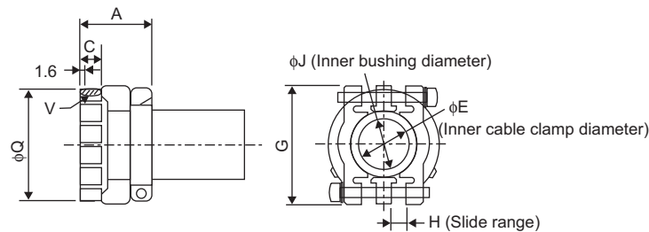
(c) MS3057A-10A: Cable Clamp with Rubber Bushing
