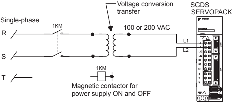
Single-phase Power Supply Connection Example
