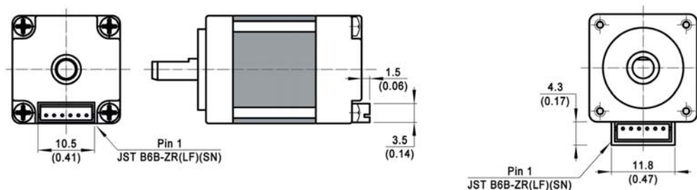
Rear facing "R" connector detail
