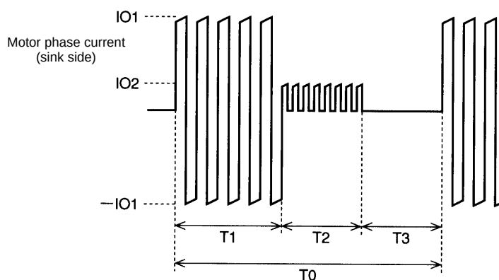
Figure 3 Motor Current Timing
