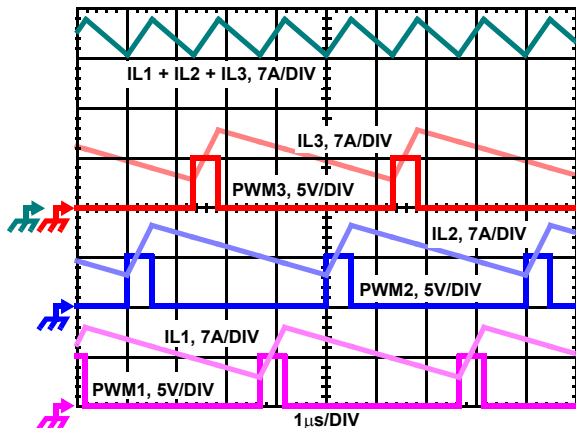
FIGURE 1. PWM AND INDUCTOR-CURRENT WAVEFORMS
