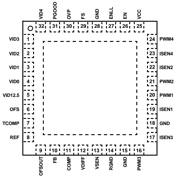
32 LEAD QFN TOP VIEW
