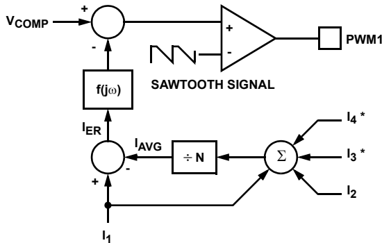
FIGURE 4. CHANNEL-1 PWM FUNCTION AND CURRENT-BALANCE ADJUSTMENT
