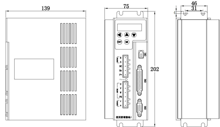
Figure 1 Drive mounting dimensions drawing
