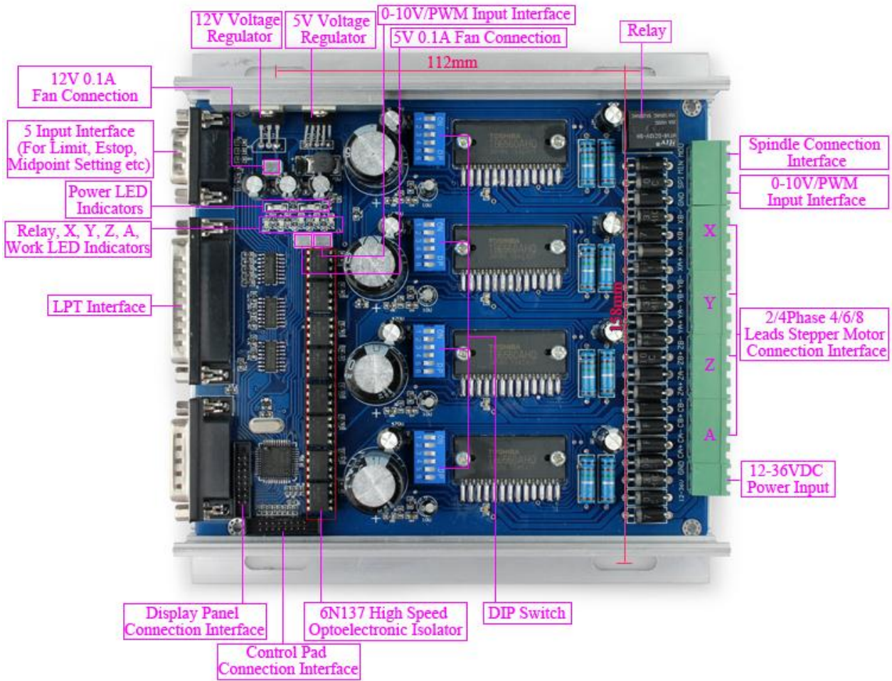
Figure 1: PCB Instructions & Specifications
