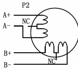
Figure 8: 6-lead motor full coil (higher torque) connections
