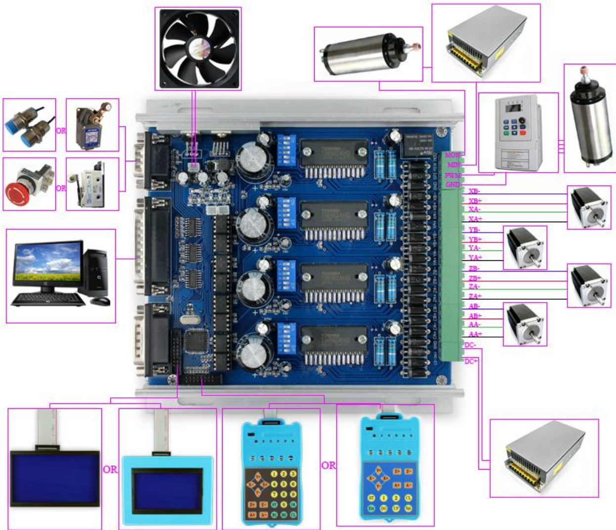
Figure 12: Wiring Diagram
