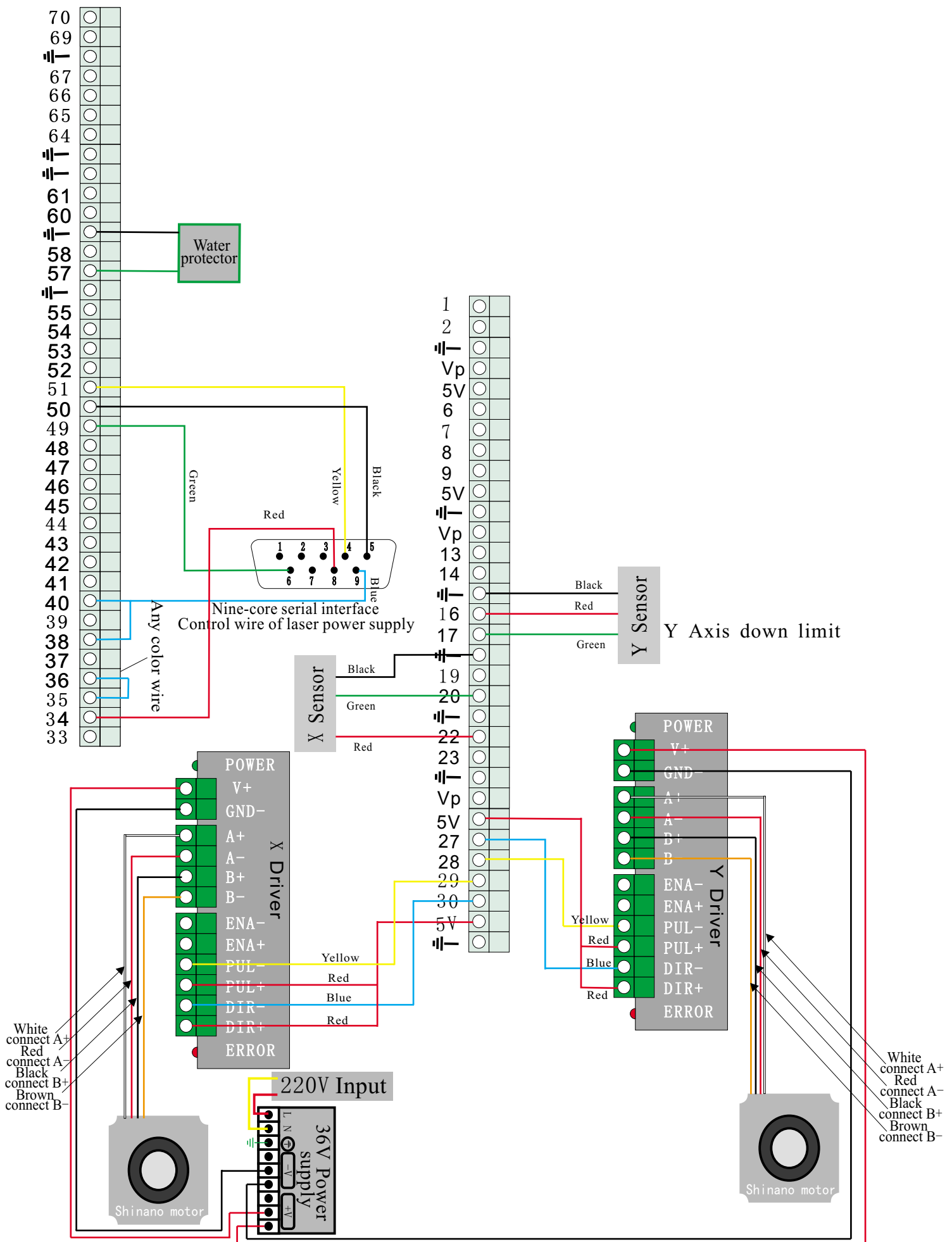
Ver 2.0/Ver2.2 Wire connection diagram for Shinano electromotor
