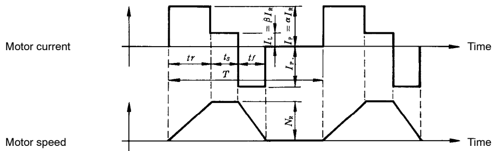
Figure 3.3 Motor Current – Motor Speed Timing Chart
