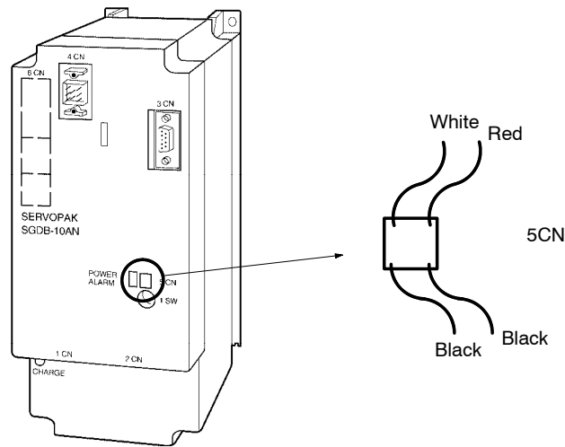
Figure 5.10 Enlarged View of the 5CN Section
