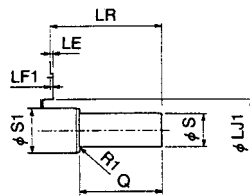
Shaft Extension (SGMG-03A2B to 09A2B)
