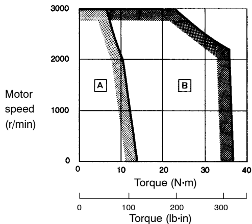
SGMD-22A□AAB
