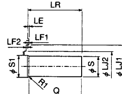
Shaft Extension (SGMG-20ASAAB to 44ASAAB)
