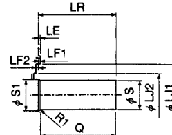
Shaft Extension (SGMG-12ASB to 60ASB)
