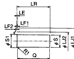
Shaft Extension (SGMG-20A2A to 75A2A)
