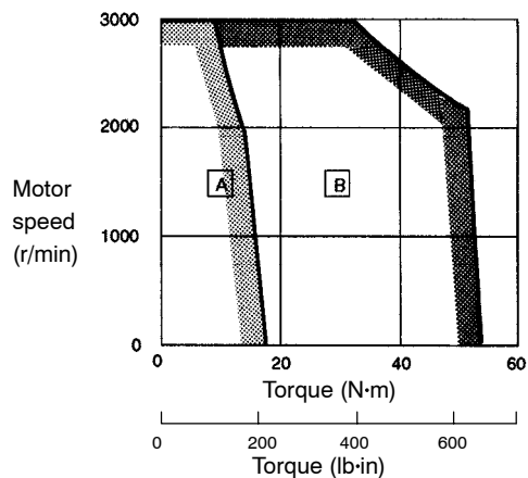
SGMD-32A□AAB
