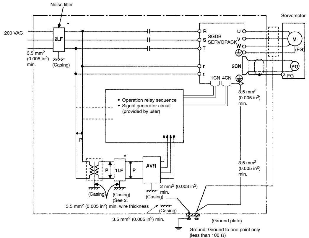
Figure 5.4 Grounding
