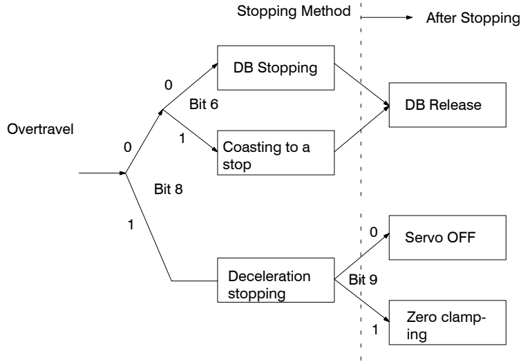
Stop Sequence in the Overtravel (OT)
