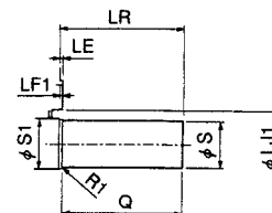
Shaft Extension (SGMG-1AASAAB)
