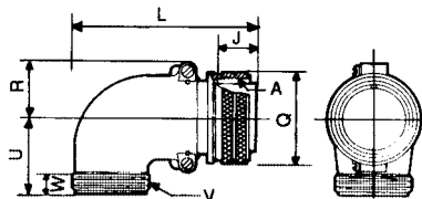
MS3108B L-shaped Plug Shell
