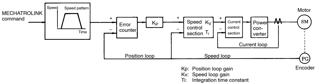
Figure 5.9 Servo System Block Diagram
