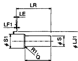
Shaft Extension (SGMG-03ASBAB to 09ASBAB)
