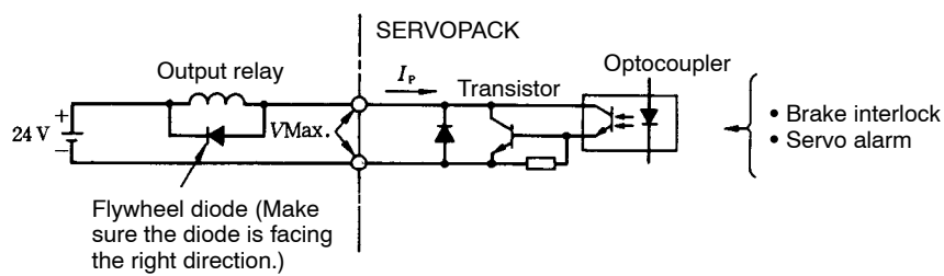
Figure 4.6 Output Circuits
