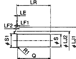
Shaft Extension (SGMG-12A2BAB to 30A2BAB)
