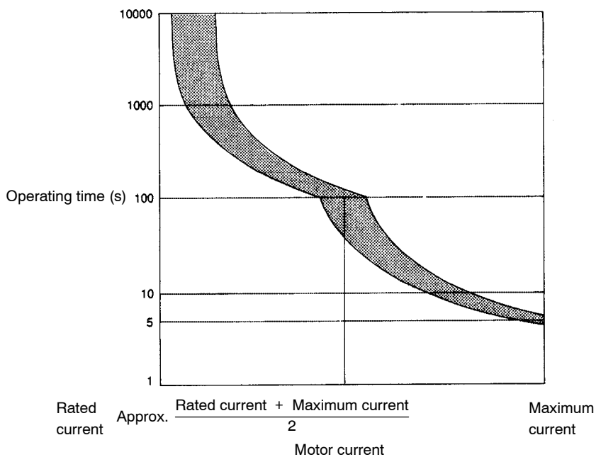
Figure 3.1 Overload Characteristics
