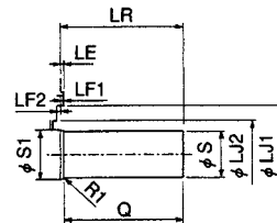
Shaft Extension (SGMG-12A2B to 60A2B)
