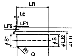
Shaft Extension (SGMG-12ASBAB to 30ASBAB)
