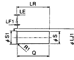
Shaft Extension (SGMG-1AA2AAB)
