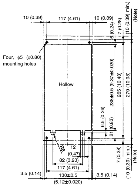
View of the Mounting Surface
