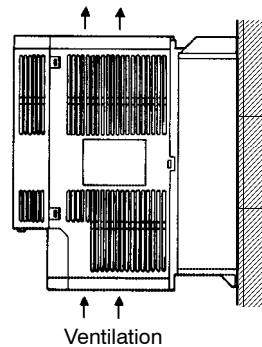
Figure 8.3 Installation Orientation
