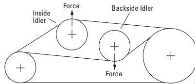
Fig. 23 Idler Forces
