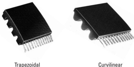
Fig. 14 Belt Construction
